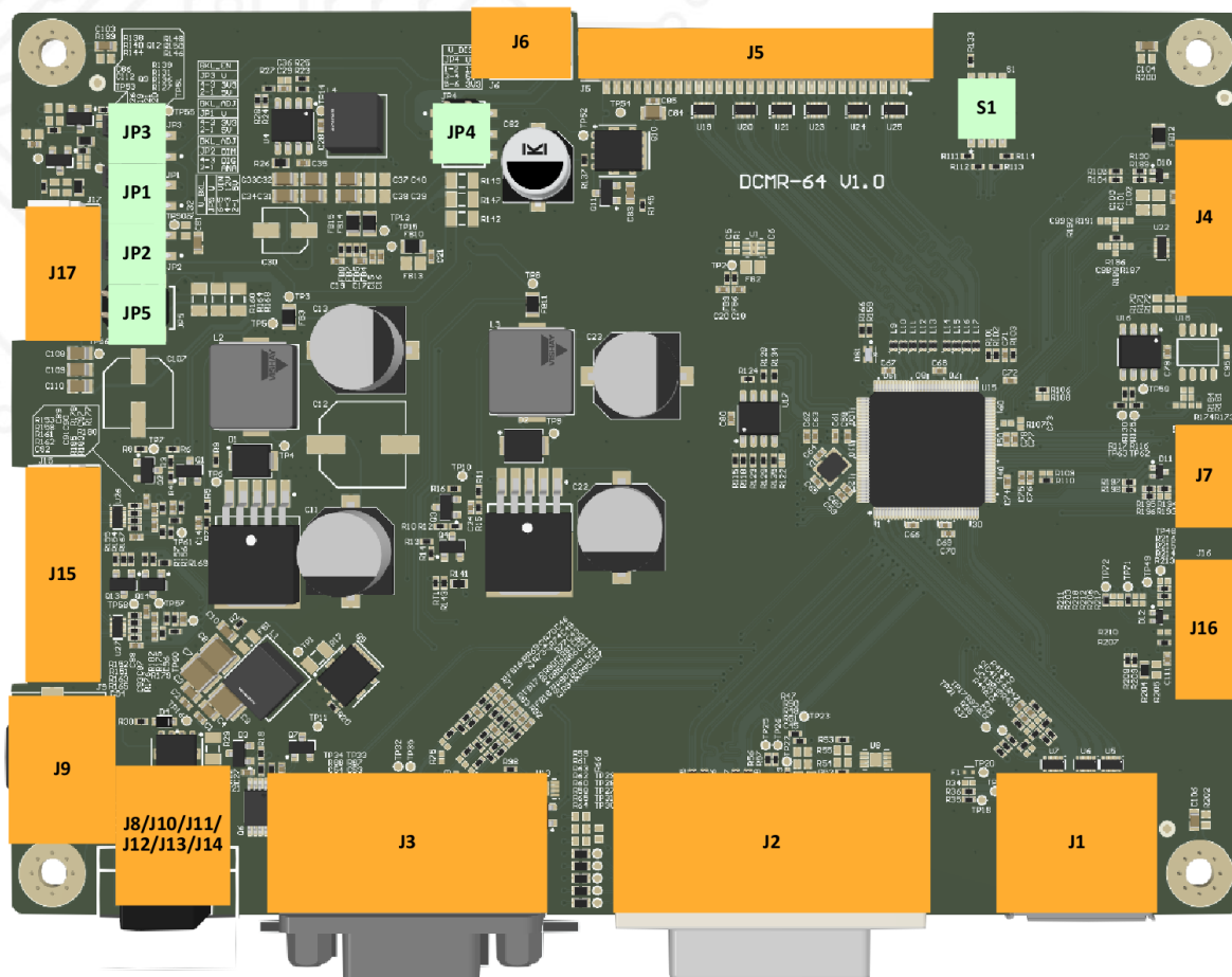
Figure 2. Board overview
